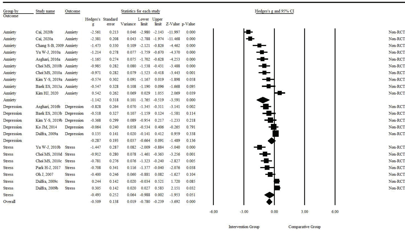
Supplementary Figure 3. Effects of nonpharmacological interventions in non-randomized controlled trials (non-RCT) on women with high-risk pregnancies.
